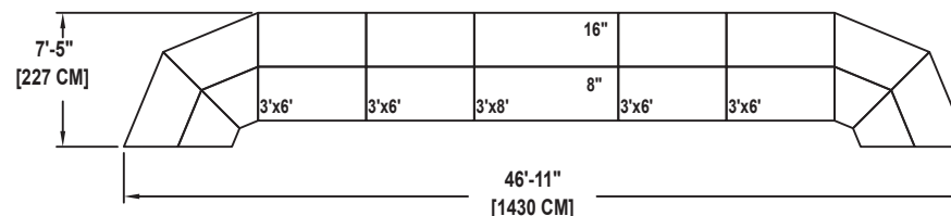
WINGED SHAPE
