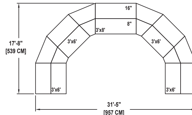
SEMICIRCLE SHAPE
