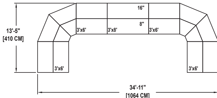
HORSESHOE SHAPE
